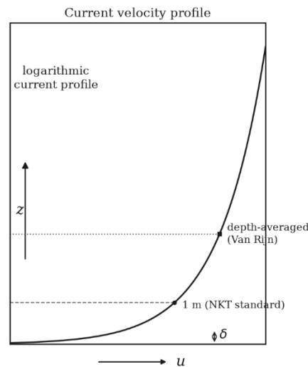
Figure 3.5: Logarithmic velocity profile of a steady current, with the reference levels used in this thesis: the NKT standard at one meter above the bed and the depth-averaged velocity at about 0.37 h that the Van Rijn method requires. The one-meter standard sits above the thin wave boundary layer and
