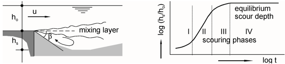
Figure 6.1: the mixing layer ( h_o , u , h_s , angle \beta ) and the four scour phases I-IV on a \log(h_s/h_o) versus \log(t) plot up to the final depth. After Schiereck and Verhagen (2019).
